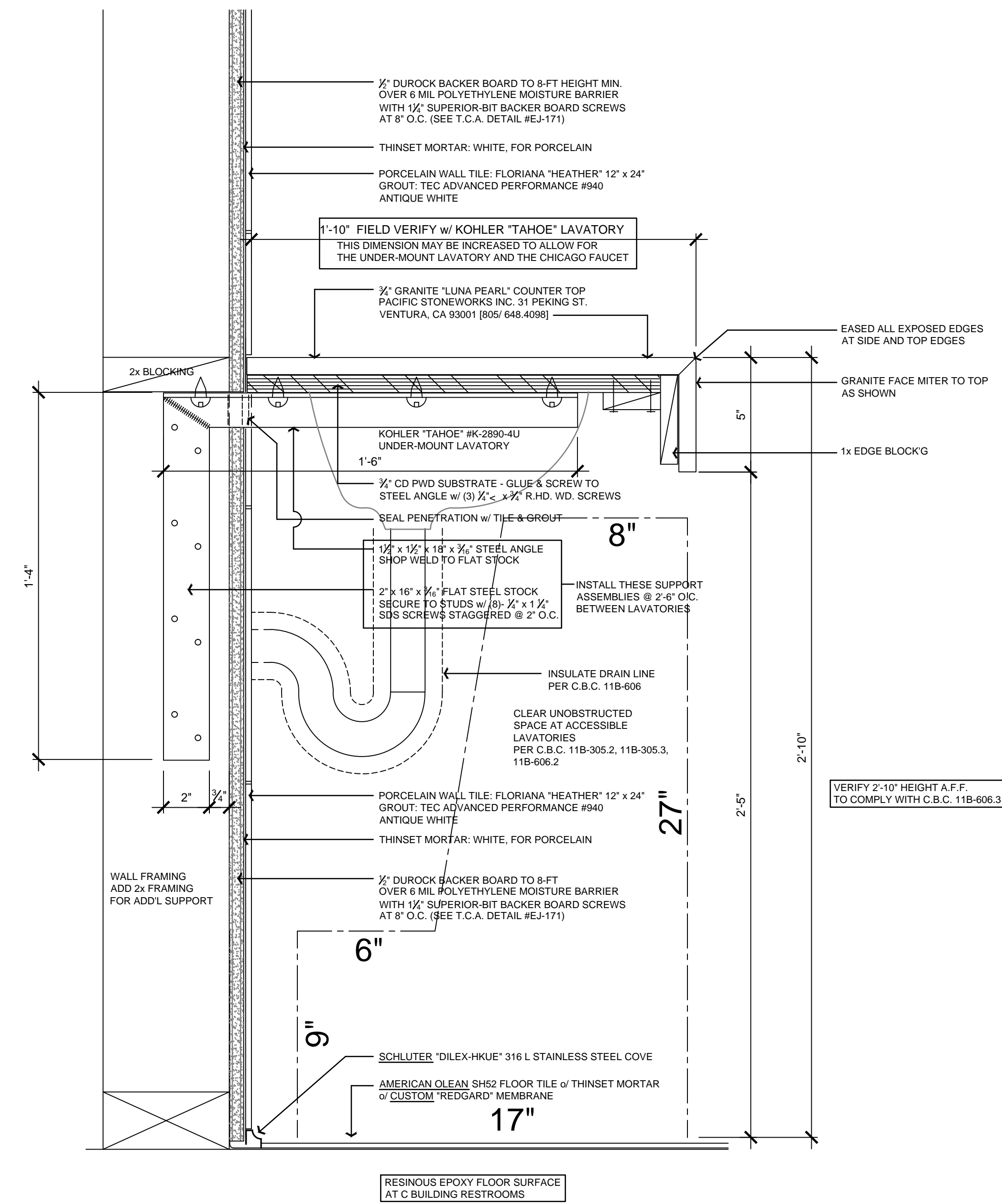
4 H.C. COUNTER TOP SUPPORT DTL - TYPICAL SCALE: 3" = 1'-0"
