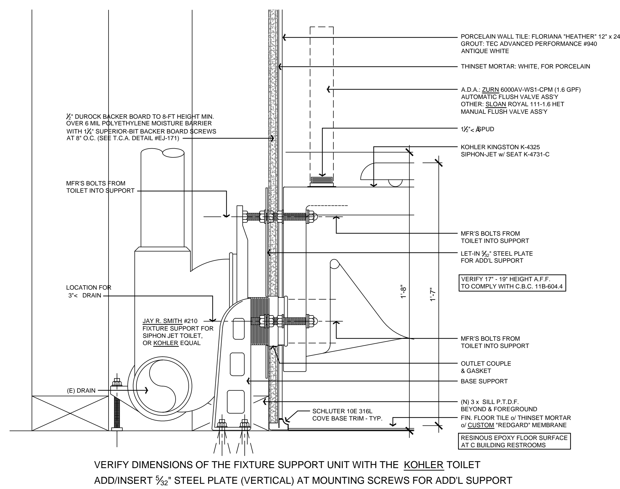
1 WALL HUNG TOILET FIXTURE SUPPORT - TYPICAL SCALE: 3" = 1'-0"
