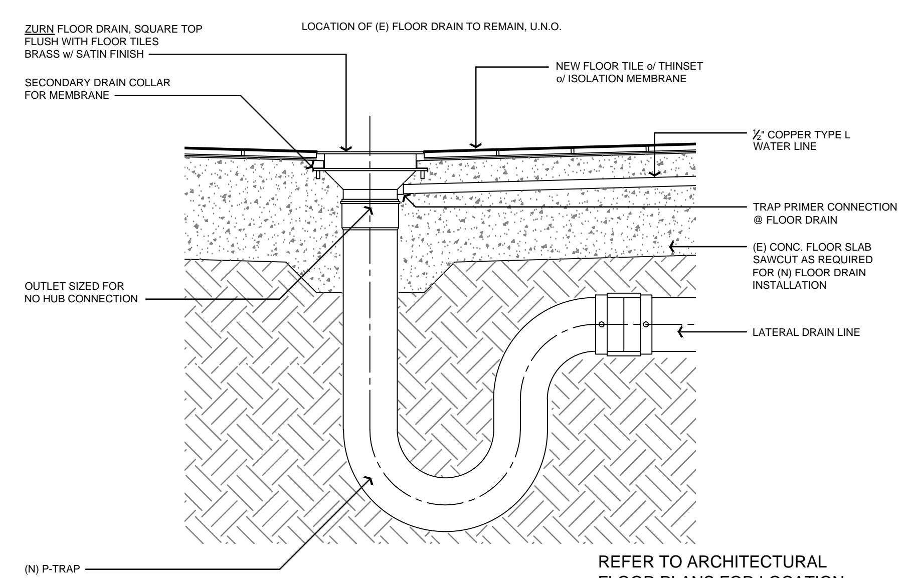
3 FLOOR DRAIN DETAIL SCALE: 3" = 1'-0"
