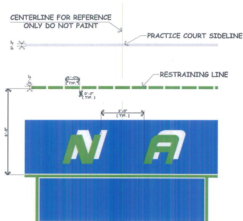
3 ENLARGED END COURT DETAIL NTS
