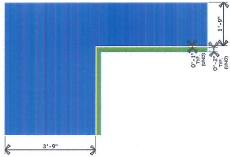
1 COURT LINES @ CORNERS NTS
